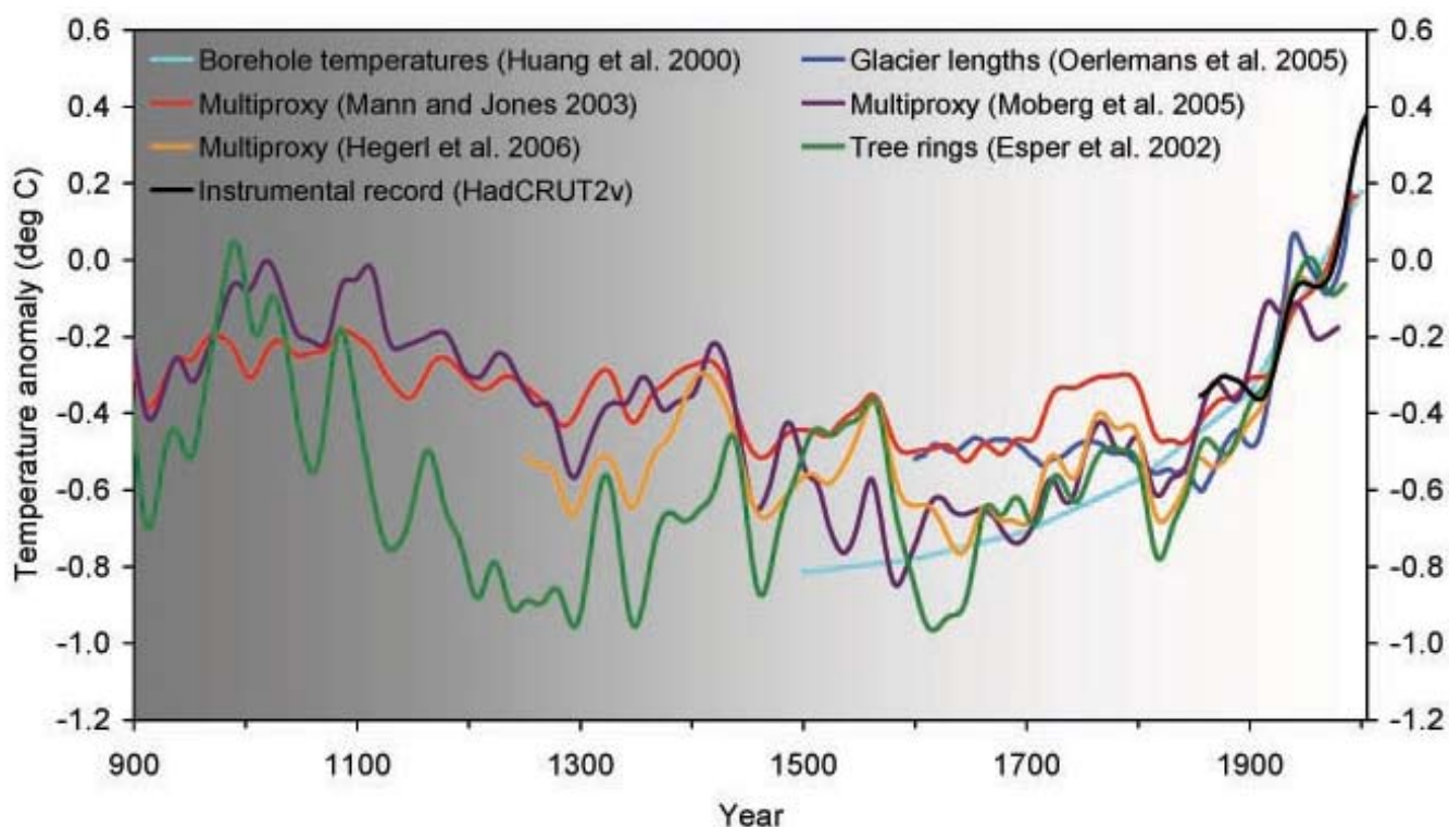
Figure S-1. Smoothed reconstructions of large-scale (Northern Hemisphere mean or global mean) surface temperature variations from six different research teams are shown along with the instrumental record of global mean surface temperature. Each curve portrays a somewhat different history of temperature variations, and is subject to a somewhat different set of uncertainties that generally increase going backward in time (as indicated by the gray shading). This set of reconstructions conveys a qualitatively consistent picture of temperature changes over the last 1,100 years, and especially the last 400.
