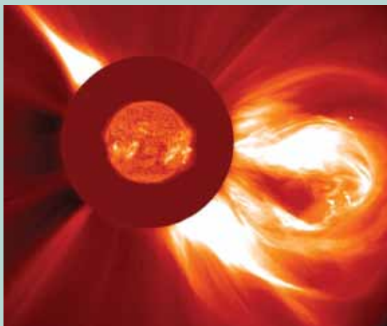
Figure 6. A composite image from the Solar & Heliospheric Observatory satellite showing a coronal mass ejection blasting out into space. Such events produce environmental changes termed “space weather.” Source: NASA
