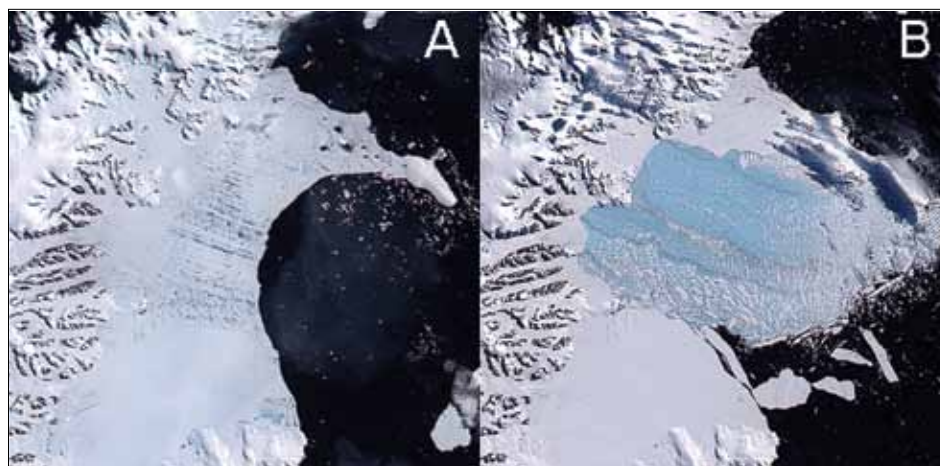
Figure 1. The Larsen Ice Shelf extends along the east coast of the Antarctic Peninsula (Image A). In 2002, the Larsen B ice shelf suddenly collapsed, delivering 3,250 km 2 of ice into the ocean (Image B). Better predictions of the effects of warming climate on ice shelves could help prevent similar occurrences from being surprises in the future.
